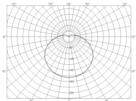
LUMINOUS INTENSITY (cd/1000lm)
