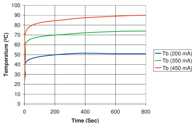
Figure 5: MCPCB Temperature
