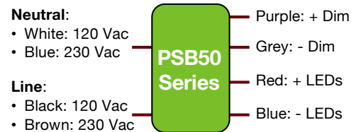
Wiring Diagram
