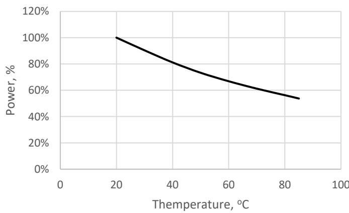
Fig 5. Relative Radiant Flux vs Ambient Temperature
